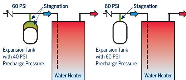
FIGURE 2 Older Style, Dead-end Thermal Expansion Tank with Pre-Charge Less Than System Pressure – Allows Stagnant Water Storage.
