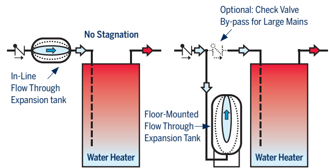
FIGURE 4 In-Line, Flow-Through Thermal Expansion Tank
